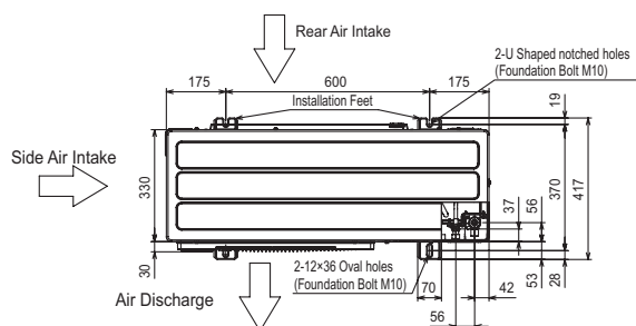
MXZ-8B140VA/YA, MXZ-8B160VA/YA
